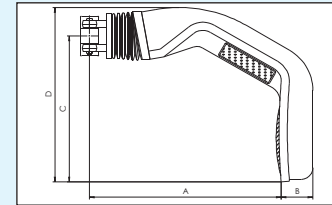
A=1000mm, B=160mm, C=620mm, D=720mm Rear view mirror : 365 x 190 Down view mirror : 190 x 140
